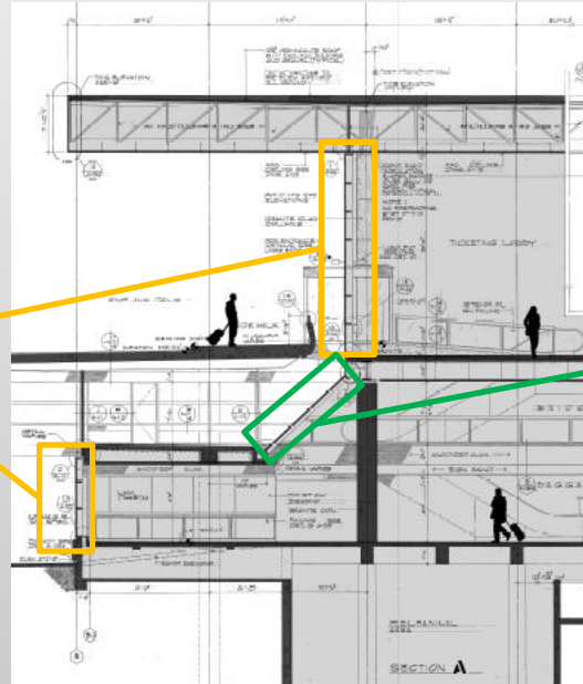
Main Terminal Cross-Section
